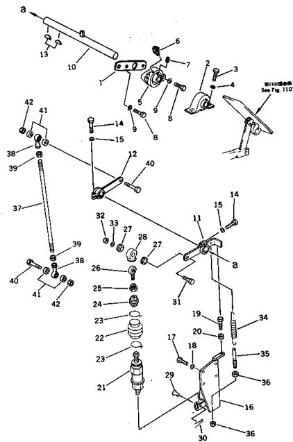
FIG. 1102 FUEL CONTROL LINKAGE (2/2)
