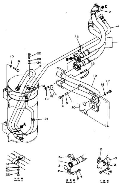
Fig. 102A BYPASS FILTER PIPING (Serial No. 1240~)
