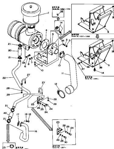
Fig. 105 AIR CLEANER AND PIPING, FRONT
