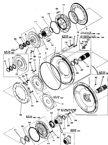
Fig. 101 ENGINE RELATED PARTS
