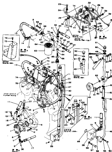
Fig. 103A PTO LUB. OIL PIPING AND FILTER (Serial No. 1084-)
