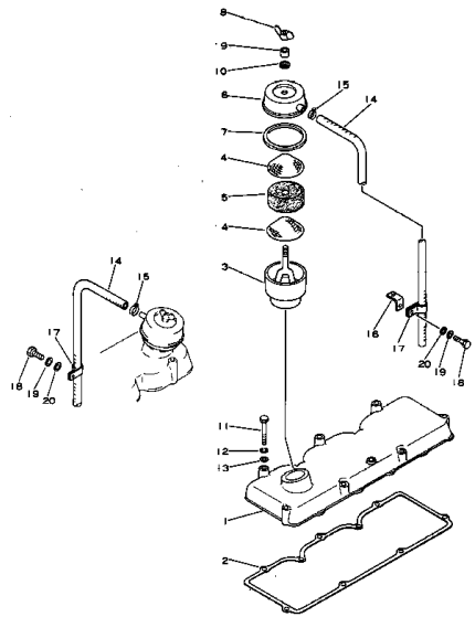
Fig. 105 ROCKER ARM HOUSING COVER (適用機種 Engine No. 430077~535023)
