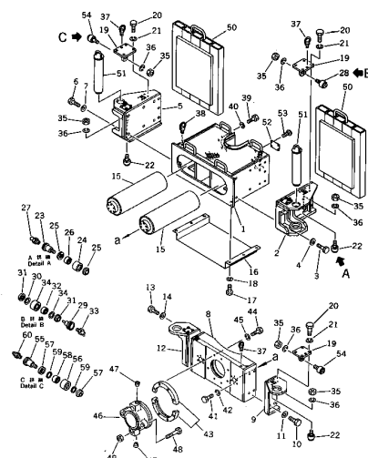
FIG. 1011A JACK AND ADAPTER (1/2) (SERIAL NO. 1267 -)
