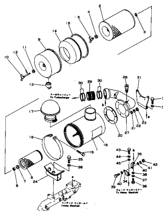
FIG. 161 AIR CLEANER
