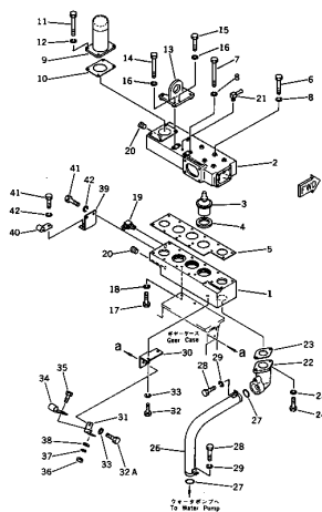
FIG. 135 THERMOSTAT AND HOUSING
