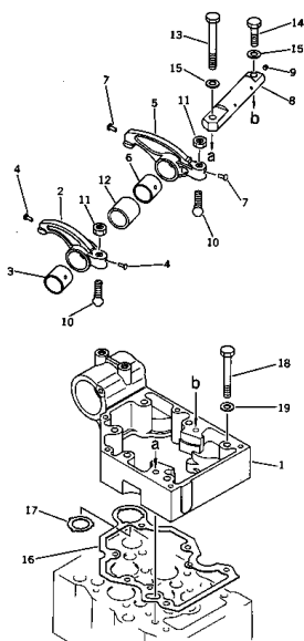
FIG. 103 ROCKER ARM AND HOUSING
