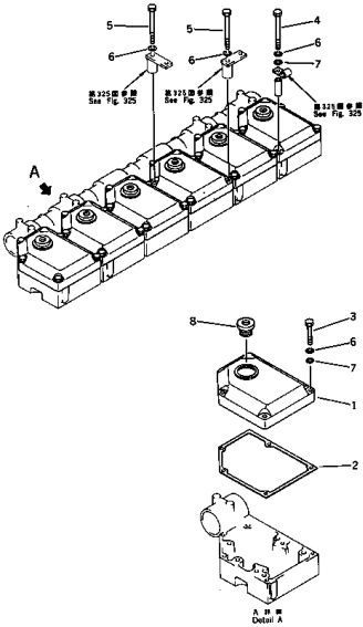
FIG. 105 ROCKER ARM HOUSING COVER
