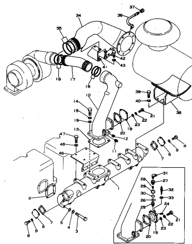
FIG. 1113A AIR INTAKE MANIFOLD AND CONNECTION (ENGINE NO. 28770-)
