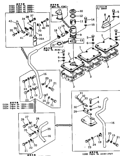
FIG. 1105 ROCKER ARM HOUSING COVER
