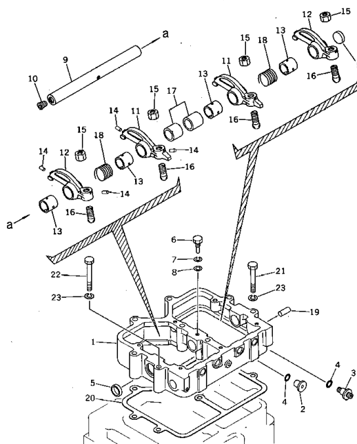
FIG. 1101 ROCKER ARM AND HOUSING
