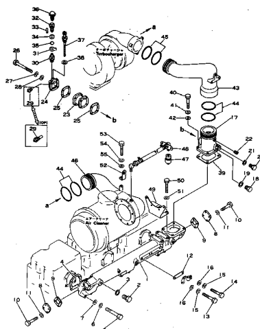
FIG. 1113 AIR INTAKE MANIFOLD AND CONNECTION
