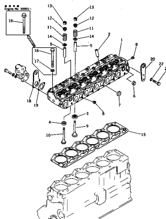
FIG. 101 CYLINDER HEAD
