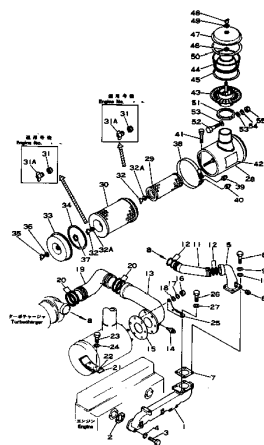
FIG. 114 AIR INTAKE MANIFOLD AND AIR CLEANER (S4D120-11C ENGINE NO. 89595-)
