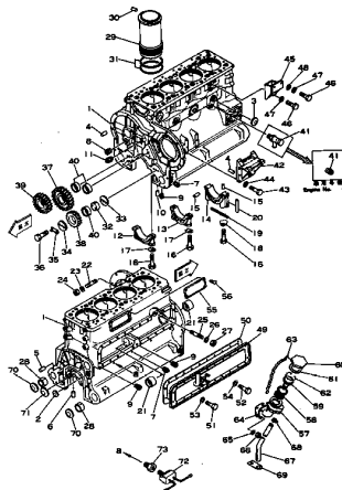
FIG. 202 CYLINDER BLOCK
