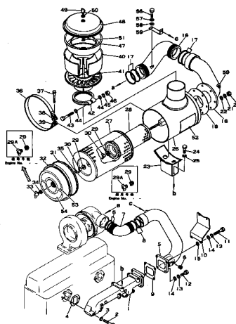
FIG. 113 AIR INTAKE MANIFOLD AND AIR CLEANER (S4D120-11A ENGINE NO. 84525-)
