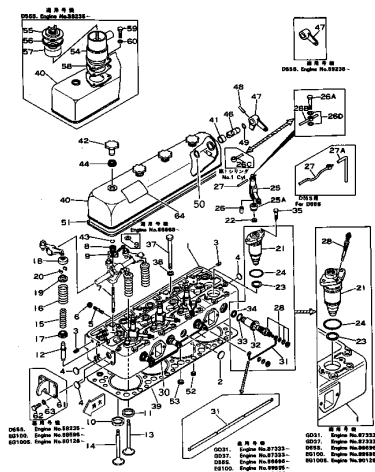
FIG. 101 CYLINDER HEAD, COVER AND PRECOMBUSTION CHAMBER
