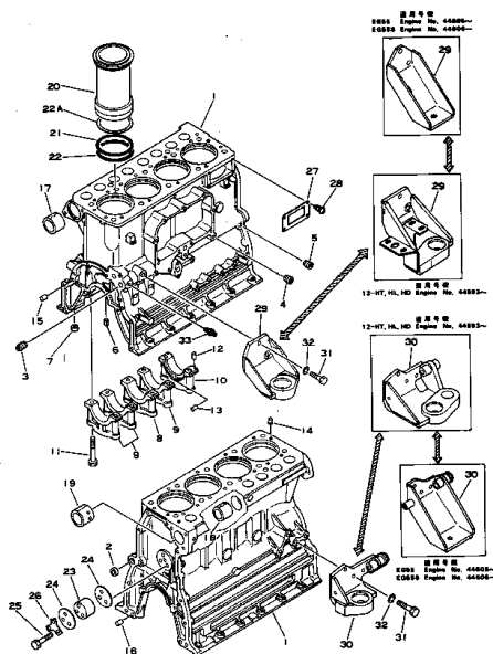
FIG. 1201 CYLINDER BLOCK
