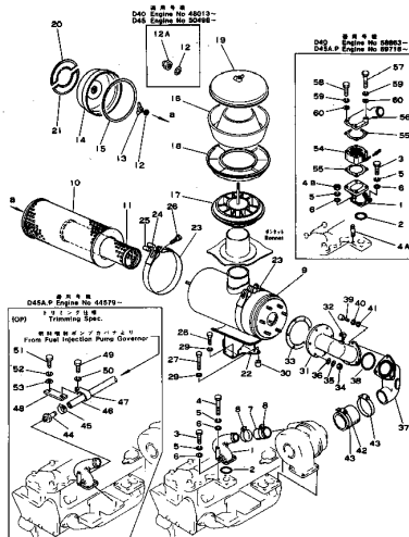
FIG. 1111 AIR INTAKE CONNECTION AND AIR CLEANER
