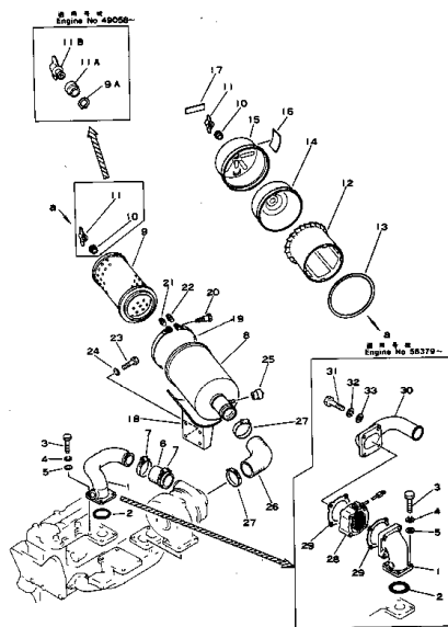
FIG. 1114 AIR INTAKE CONNECTION AND AIR CLEANER (EG55 ENGINE NO. 44605- )
