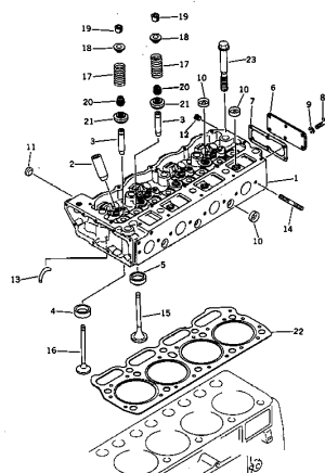
FIG. 101 CYLINDER HEAD
