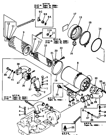
FIG. 1113 AIR INTAKE CONNECTION AND AIR CLEANER
