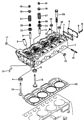
FIG. 101 CYLINDER HEAD
