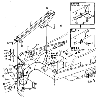
Fig. 105 YOKE (Serial No. 1001~)
