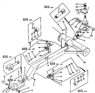
Fig. 103 DRAWBAR (Serial No. 1001~)
