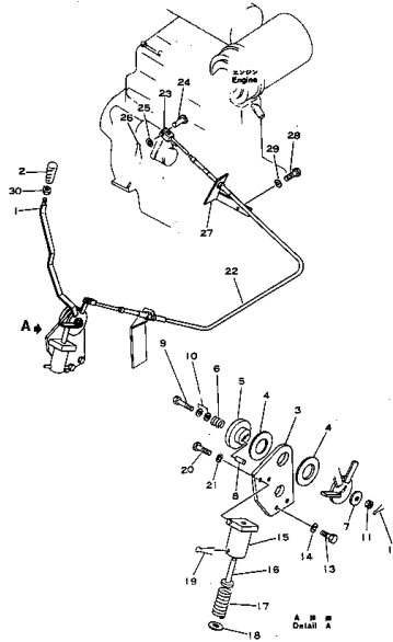
Fig. 121 FUEL CONTROL LEVER
