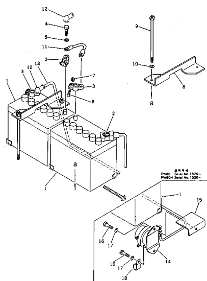
Fig. 151 BATTERY
