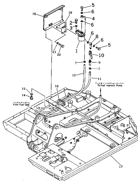
FIG-1307 追加燃料フィルタ ADDITIONAL FUEL FILTER
