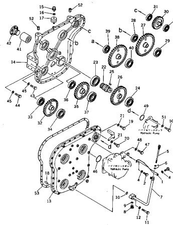
Fig. 105B POWER TAKE OFF (1/3) (PC400 Serial No. 10099-) (PC400LC Serial No. 10124-)
