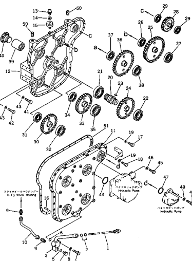
Fig. 105A POWER TAKE OFF (1/2) (PC400 Serial No. 10032~10098)
