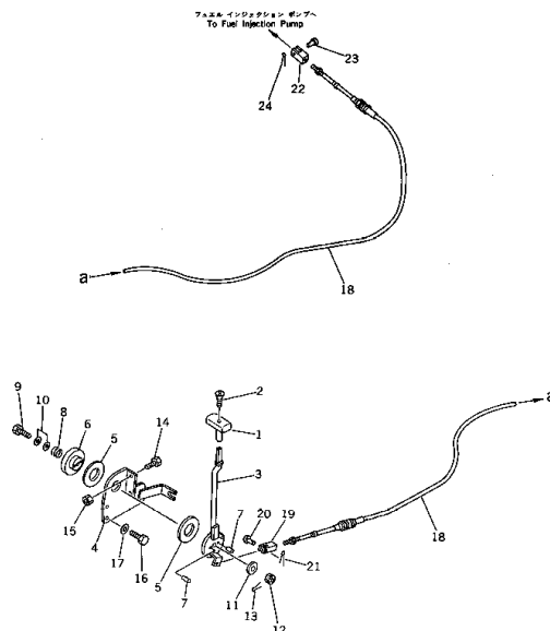
Fig. 121 FUEL CONTROL LEVER AND LINKAGE
