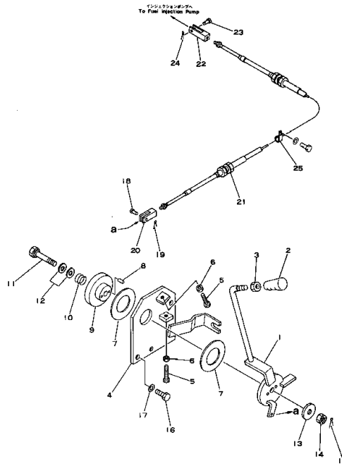
Fig. 121 FUEL CONTROL LEVER AND LINKAGE Fig. 121 FUEL CONTROL LEVER AND LINKAGE
