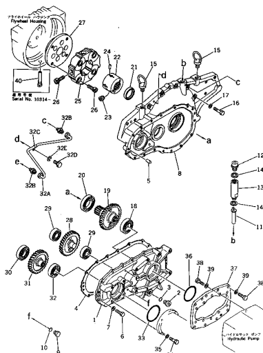
Fig. 105 POWER TAKE OFF (PC300 Serial No. 10001~10507) (PC300LC Serial No. 10001~10507)
