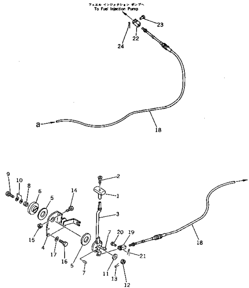
Fig. 121 FUEL CONTROL LEVER AND LINKAGE Fig. 121 FUEL CONTROL LEVER AND LINKAGE
