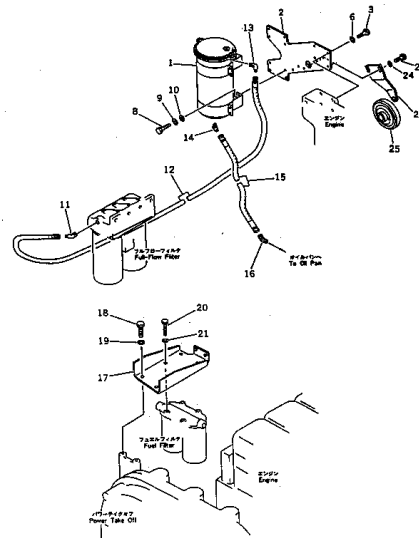
Fig. 1003 BY-PASS FILTER PIPING (For KT1150 Engine) (適用号機 (Serial No. 10001 ~ 10006))
