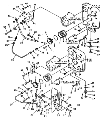
Fig. 1022 POWER TAKE OFF (5%) (For KT1150 Engine) (Serial No. 10001 )
