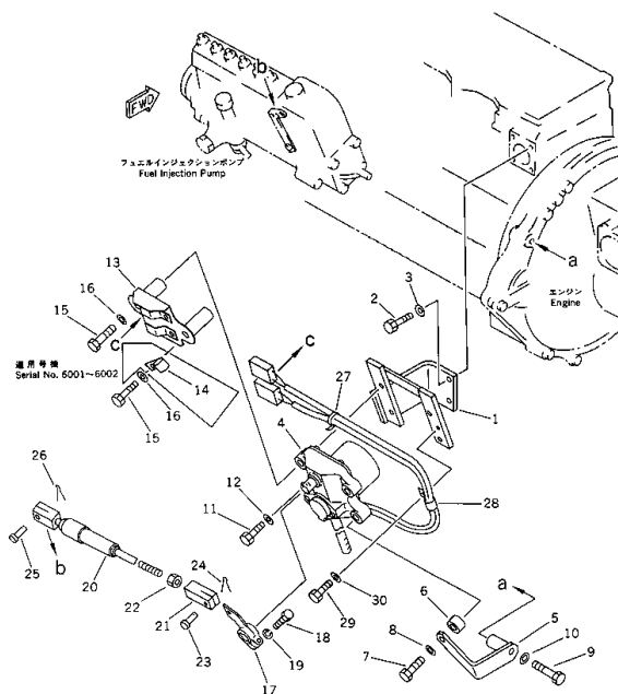
FIG. 4001 FUEL CONTROL LINKAGE (SERIAL NO. 6001-6437)
