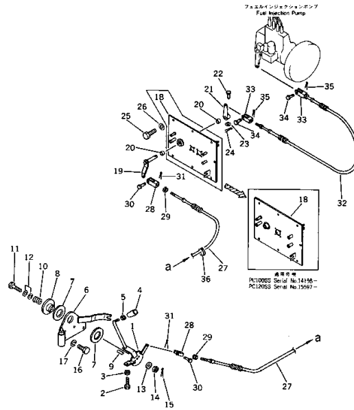
Fig. 122 FUEL CONTROL LEVER AND LINKAGE ( PC100SS Serial No. 13001 ~ ) ( PC120SS Serial No. 14001 ~ )
