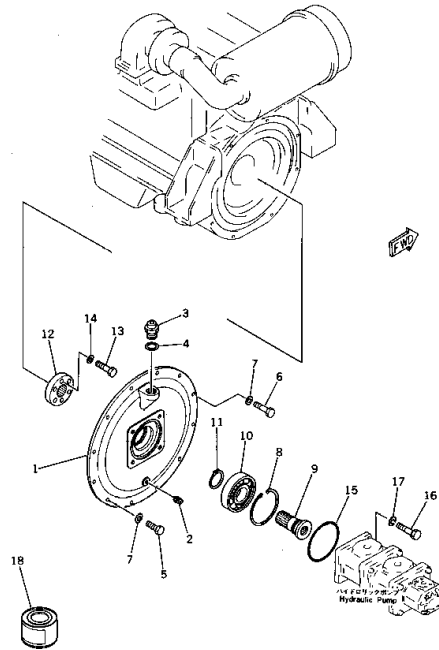
Fig. 105 POWER TAKE OFF
