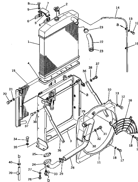
Fig. 131 RADIATOR AND OIL COOLER
