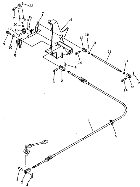
Fig. 122 FUEL CONTROL LEVER AND LINKAGE (2/2)
