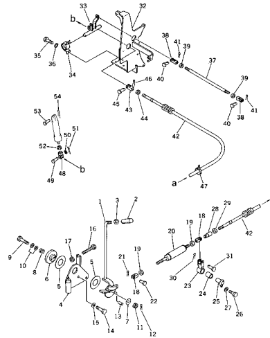
Fig. 121 FUEL CONTROL LEVER AND LINKAGE
