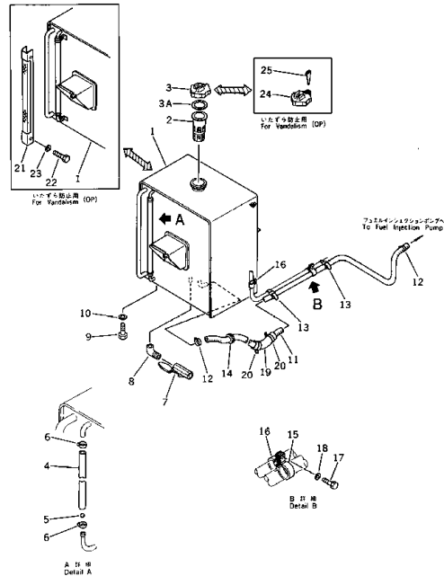
Fig. 141 FUEL TANK AND PIPING (PC100 Serial No. 13001~) (PC100L Serial No. 11001~) (PC120 Serial No. 14001~)
