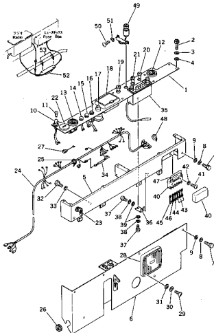
Fig. 155 INSTRUMENT PANEL PC100 Serial No. 13001-14197 PC100L Serial No. 11001-11120 PC100D Serial No. 13001-14197 PC100SS Serial No. 13001-14197 PC120 Serial No. 14001-15596 PC120SS Serial No. 14001-15596
