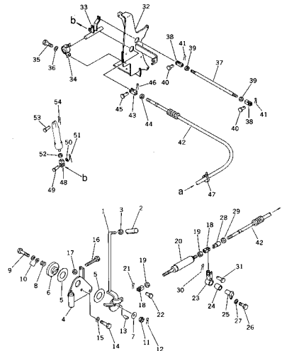
Fig. 123 FUEL CONTROL LEVER AND LINKAGE (適用機種 PC100D Serial No. 13001~)
