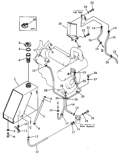
Fig. 141 FUEL TANK AND PIPING
