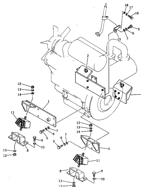
Fig. 101 ENGINE MOUNTING PARTS
