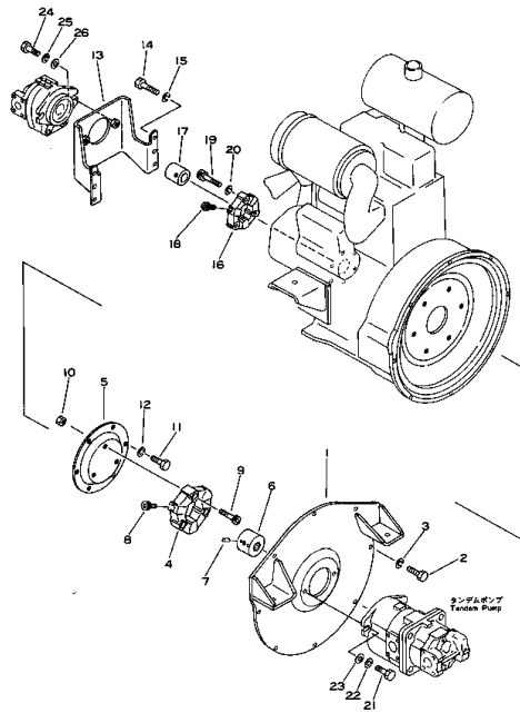
Fig. 105 POWER TAKE OFF
