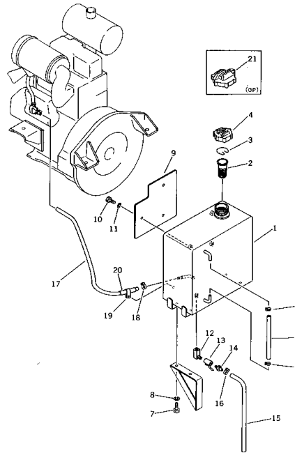
Fig. 141 FUEL TANK AND PIPING
