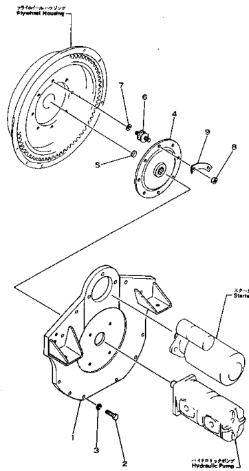
Fig. 102 POWER TAKEOFF
