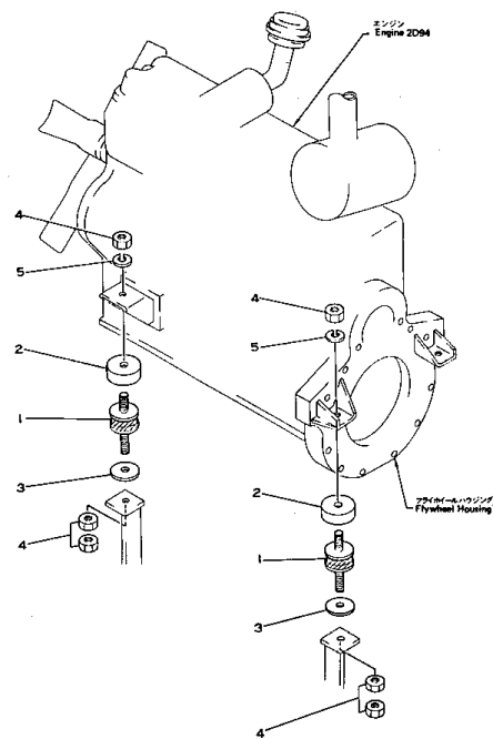
Fig. 101 ENGINE MOUNT
