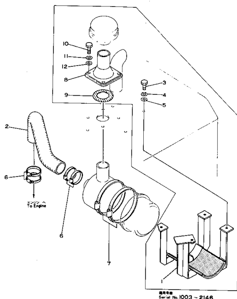
Fig. 103 AIR CLEANER CONNECTION
