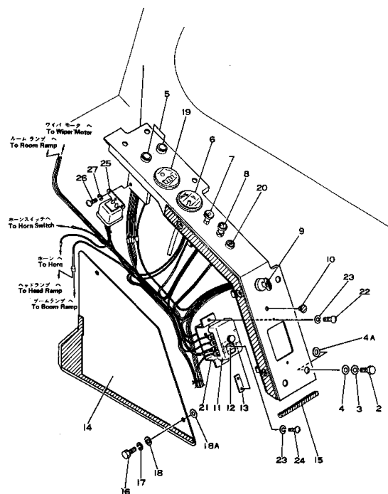
Fig. 107 INSTRUMENT PANEL
