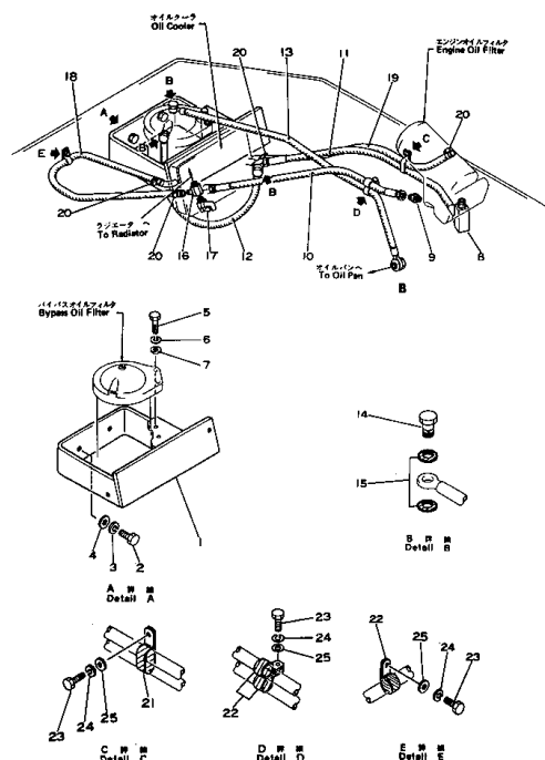
Fig. 105 ENGINE OIL COOLER PIPING (Serial No. 1003~2146)
