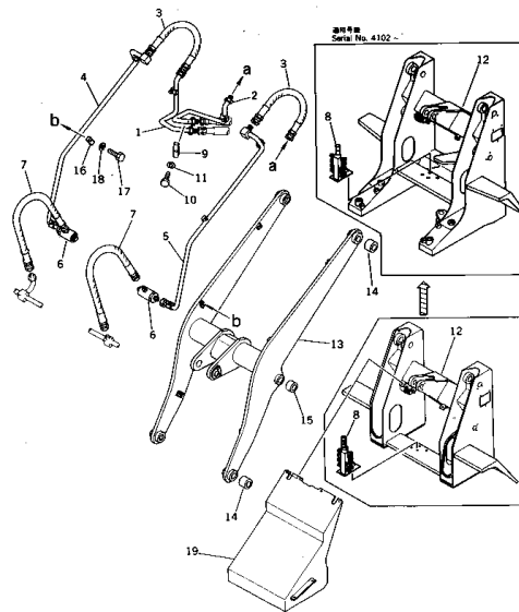
Fig. 122A HYDRAULIC PIPING (2/3) (適用 機種 (Serial No. (3001)~))
