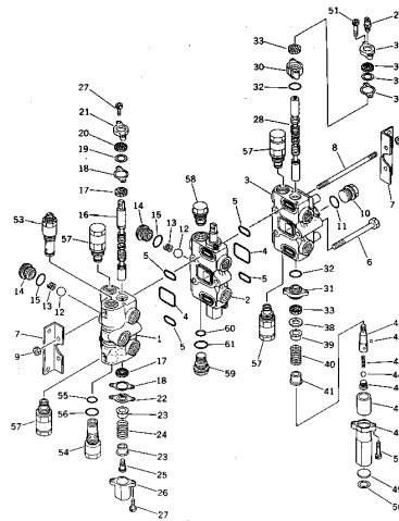
Fig. 135 HYDRAULIC CONTROL VALVE (1/2)
