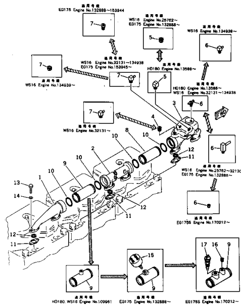
FIG. 131 WATER MANIFOLD
