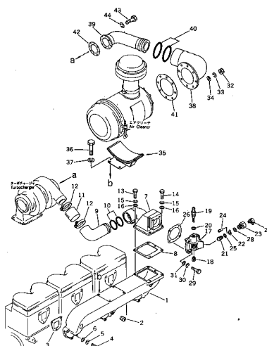
FIG. 111 AIR INTAKE MANIFOLD AND CONNECTION
