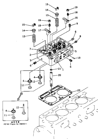
FIG. 101 CYLINDER HEAD
