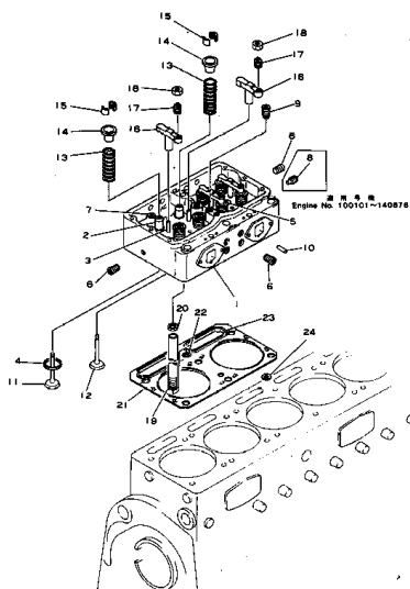
FIG. 101 CYLINDER HEAD
