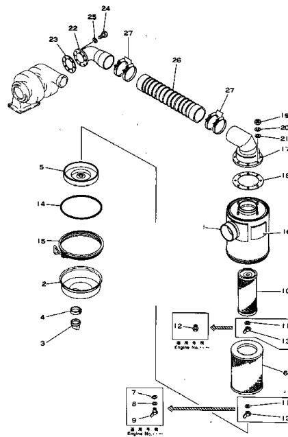
FIG. 118 AIR CLEANER AND CONNECTION
