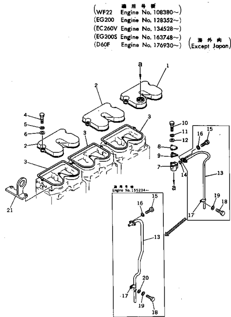
Fig. 105 ROCKER ARM HOUSING COVER
