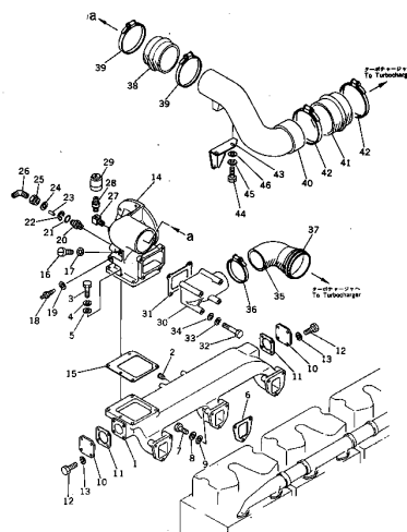
Fig. 114 AIR INTAKE MANIFOLD AND CONNECTION (EC260V Engine No. 134528~)
