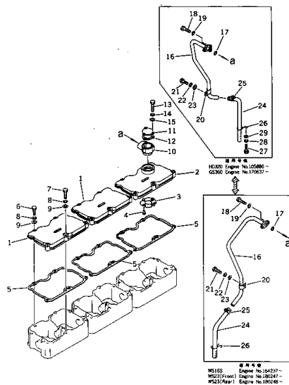
Fig. 105 RÖCKER ARM HOUSING COVER
