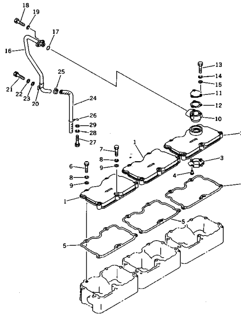
FIG. 0115 ROCKER ARM HOUSING COVER
