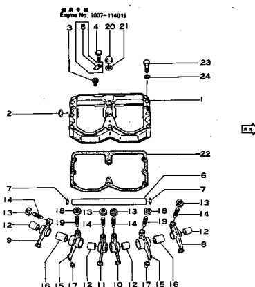
Fig. 102 ROCKER ARM AND HOUSING
