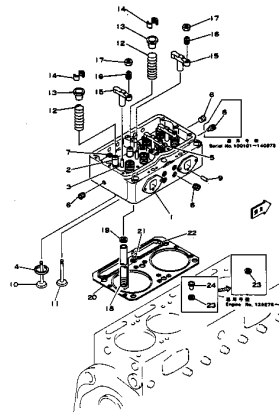
FIG. 1101 CYLINDER HEAD
