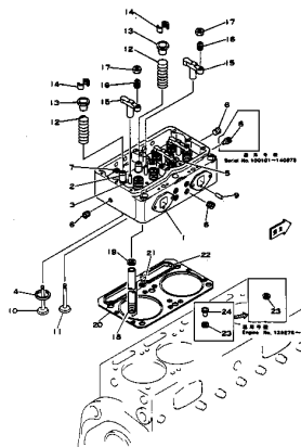
FIG. 1101 CYLINDER HEAD
