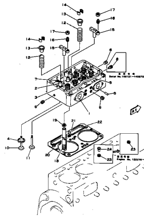
FIG. 1101 CYLINDER HEAD
