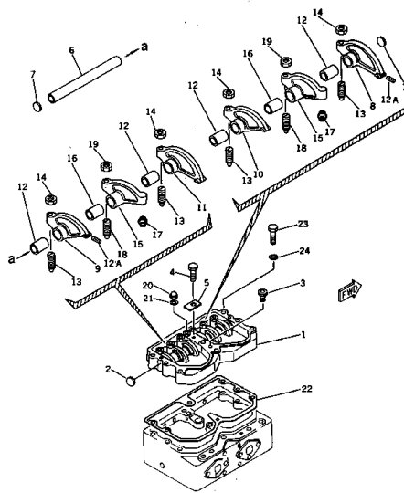
FIG. 1103 ROCKER ARM AND HOUSING
